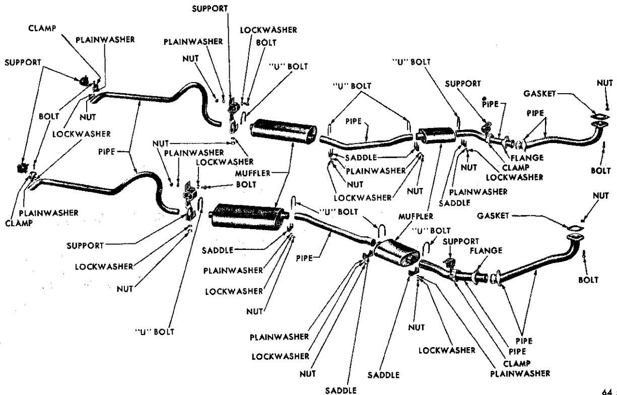
Fig. 4—Chrysler Town and Country Exhaust System
