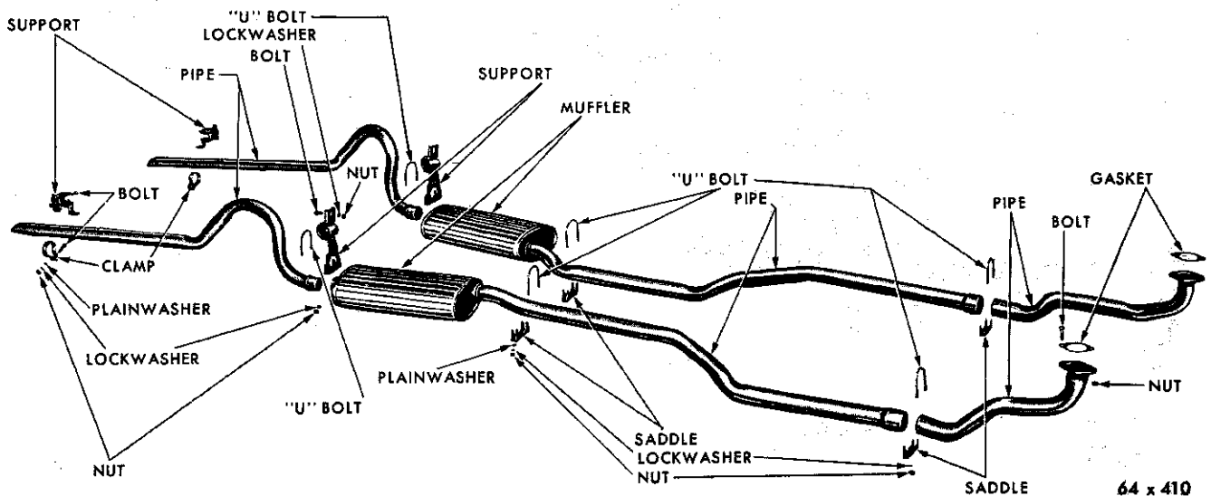
Fig. 5—Chrysler Police and High Performance Exhaust System
