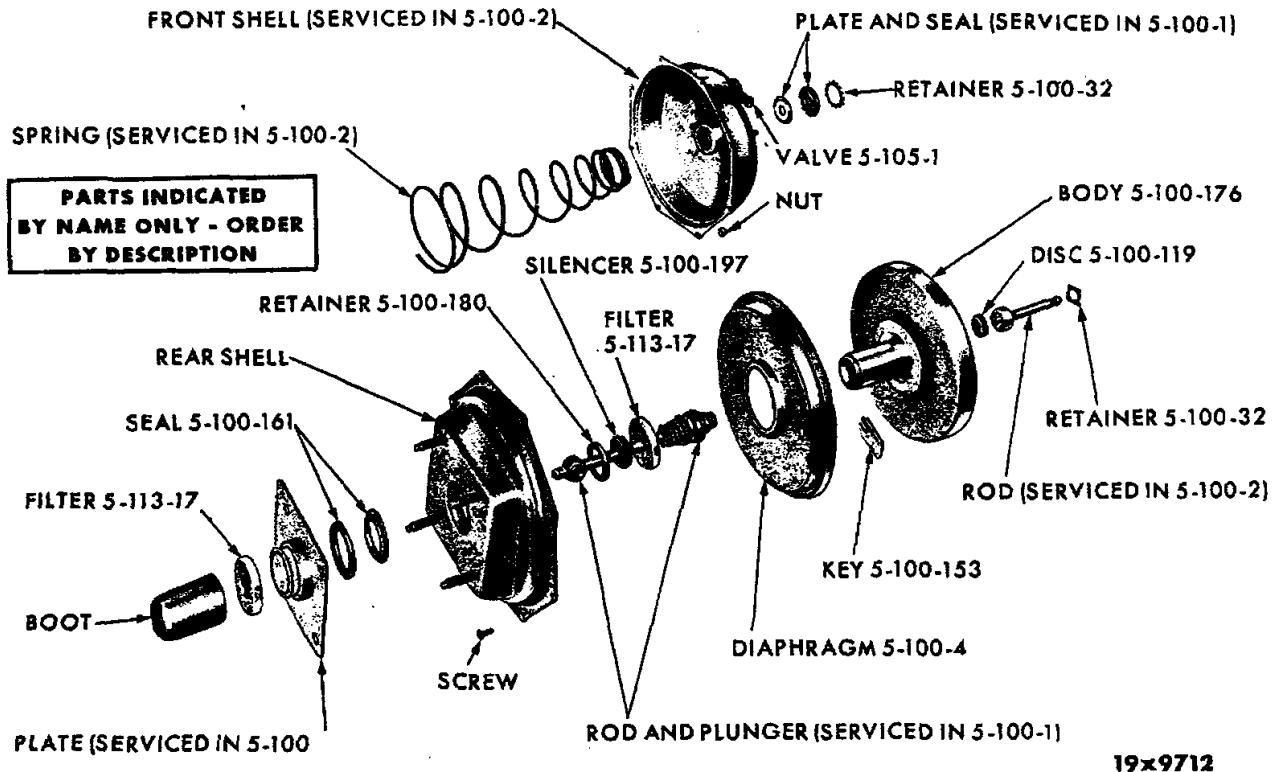
POWER BRAKE POWER UNIT - PLYMOUTH VP1-2, DODGE VD1-2, VA3, CHRYSLER VC1-2 EXCEPT VC2-300K (BENDIX TYPE)
