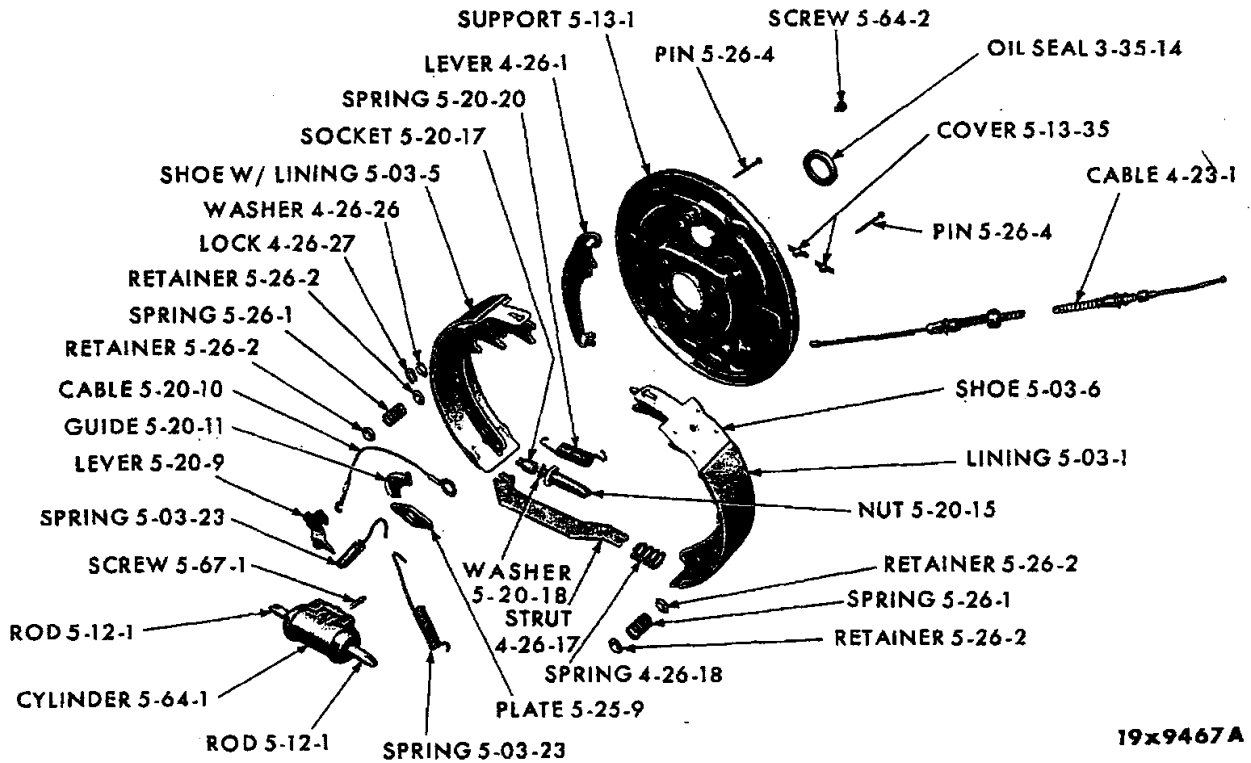
REAR WHEEL BRAKE - PLYMOUTH VP1-2, DODGE VD1-2, CHRYSLER VC1-2-3 AND IMPERIAL VY1
