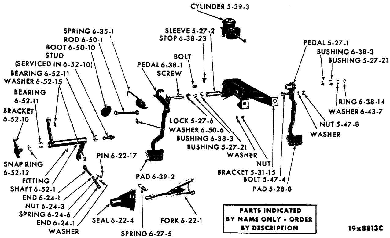
BRAKE AND CLUTCH PEDAL LINKAGE - VALIANT VV1-2 AND DART VL1-2 (WITH MANUAL TRANSMISSION)
