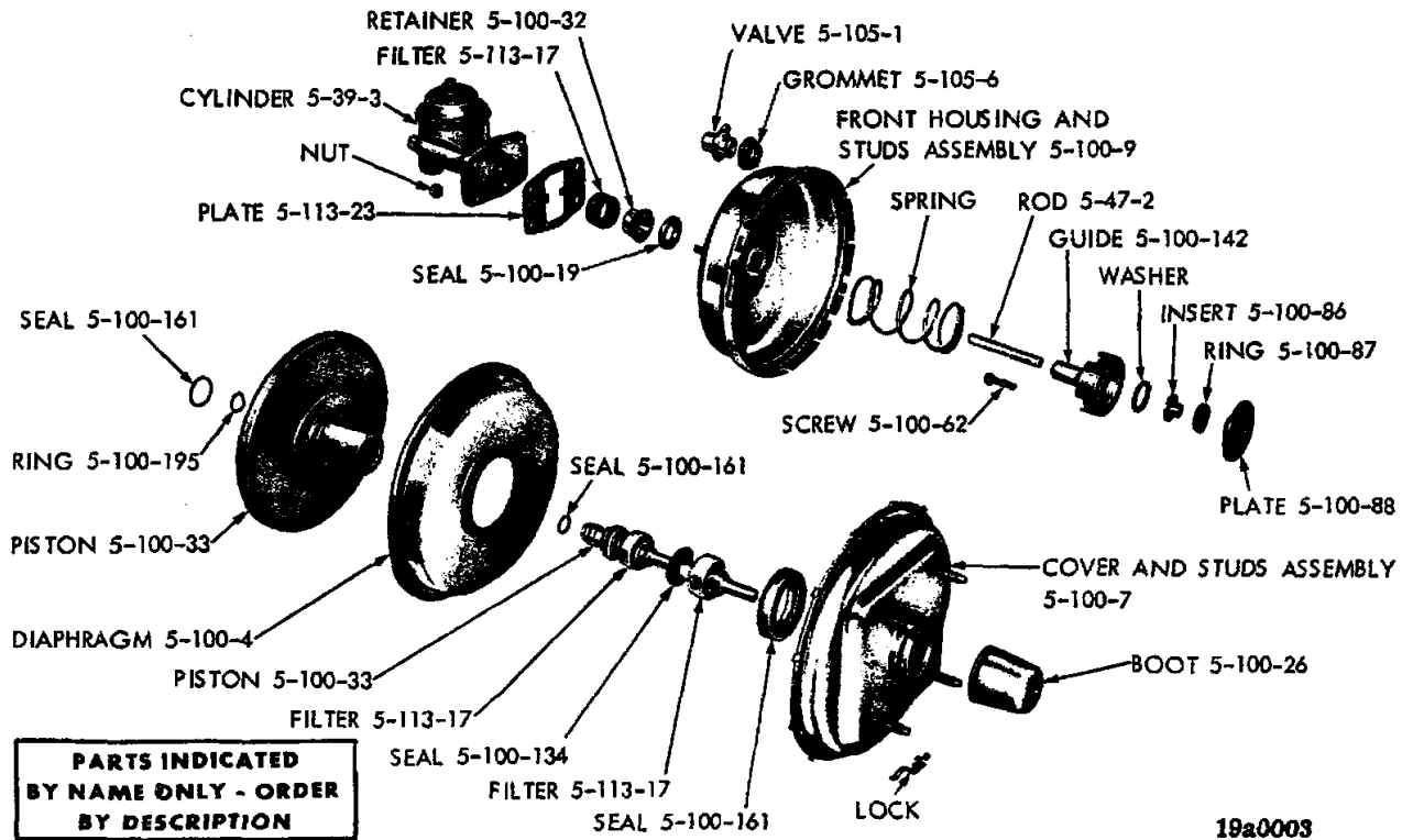
POWER BRAKE POWER UNIT - PLYMOUTH VP1-2 AND DODGE VD1-2 (KELSEY-HAYES TYPE)
