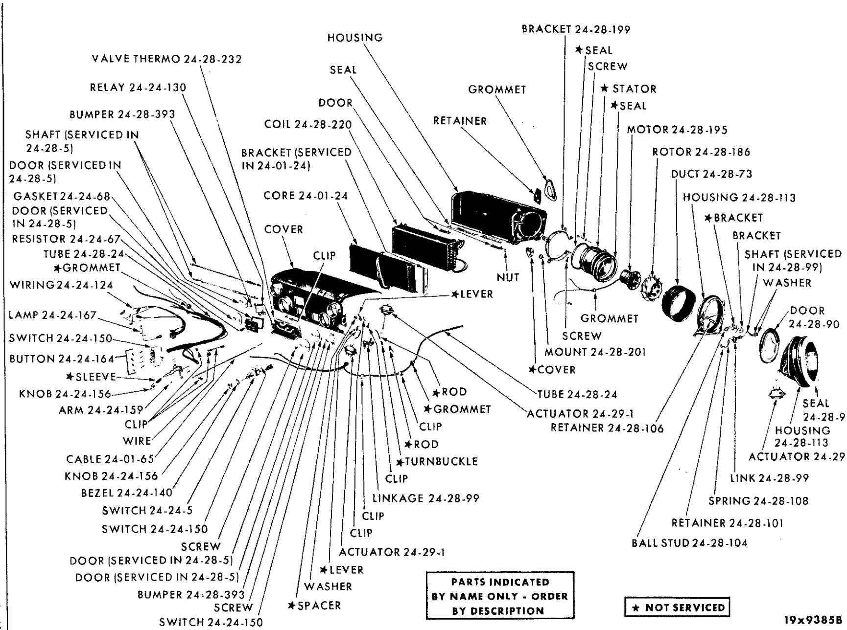
AIR CONDITIONING SYSTEM - COWL TYPE
