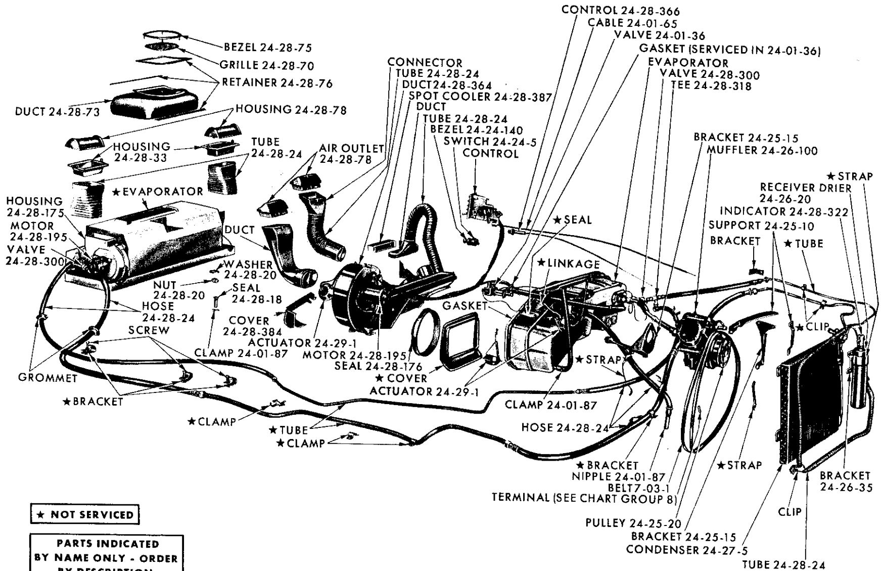
AIR CONDITIONING SYSTEM - TRUNK TYPE (DUAL)
